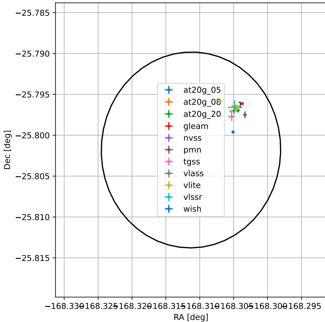
4FGL J1246.7-2548
