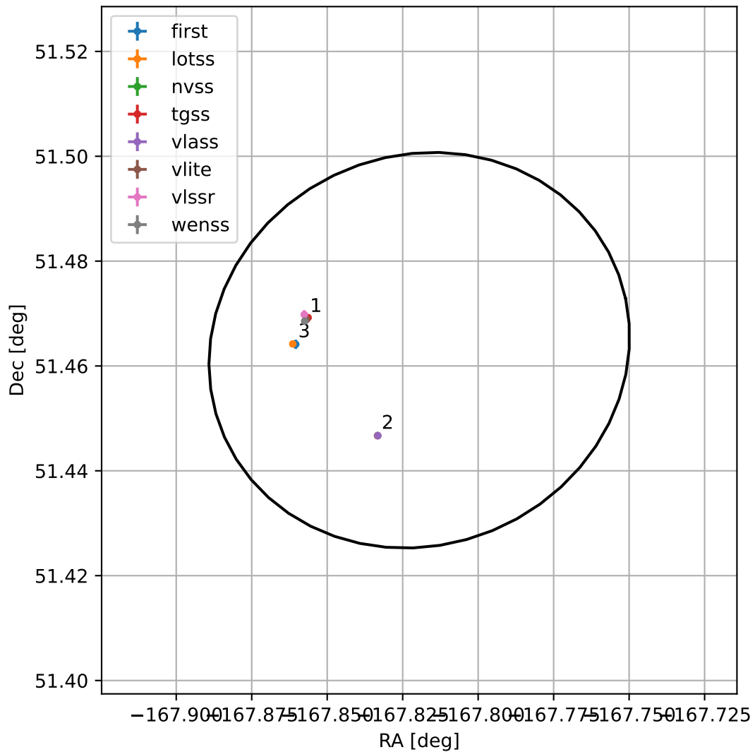
4FGL J1248.7+5127
