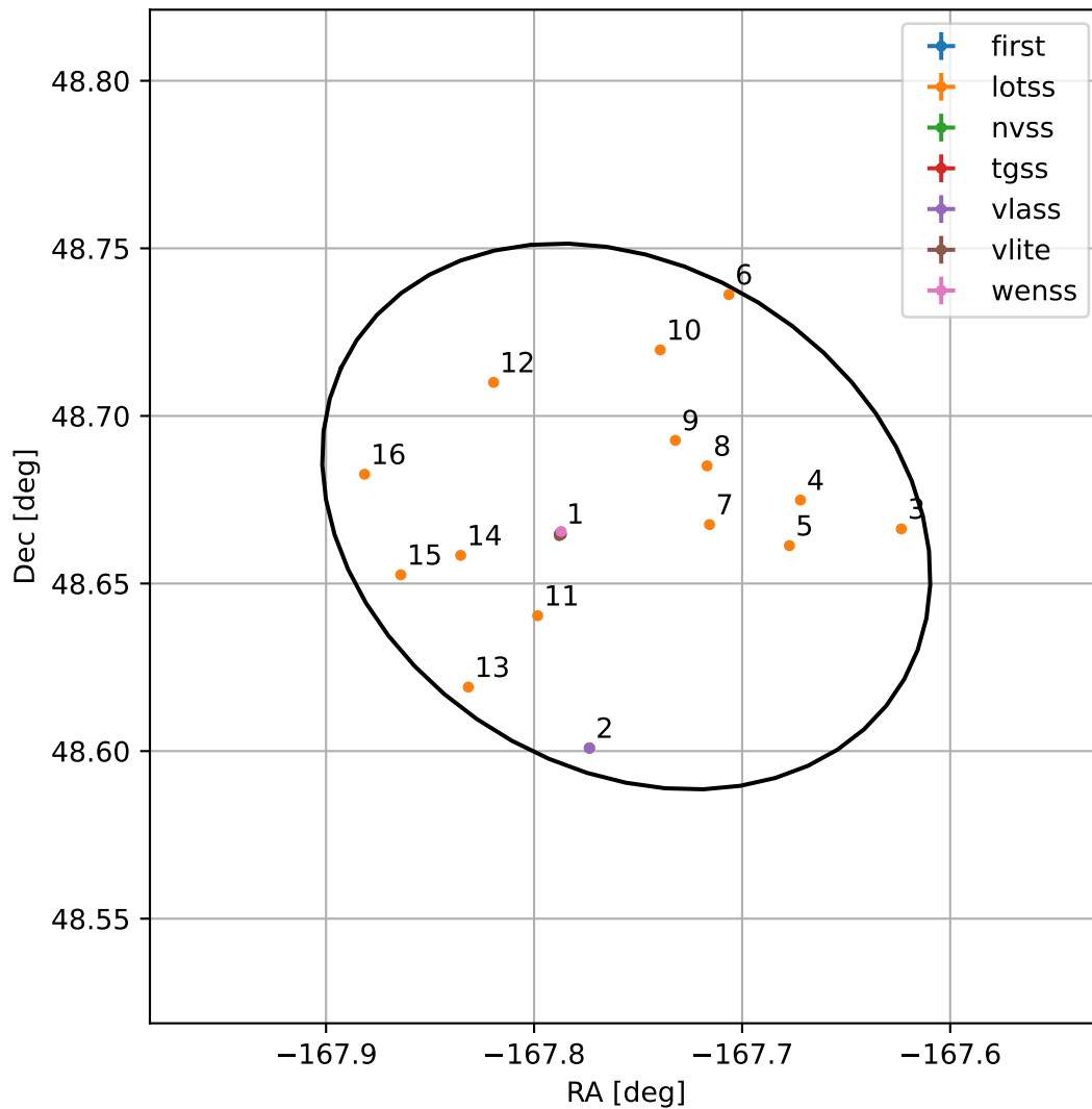
4FGL J1248.9+4840
