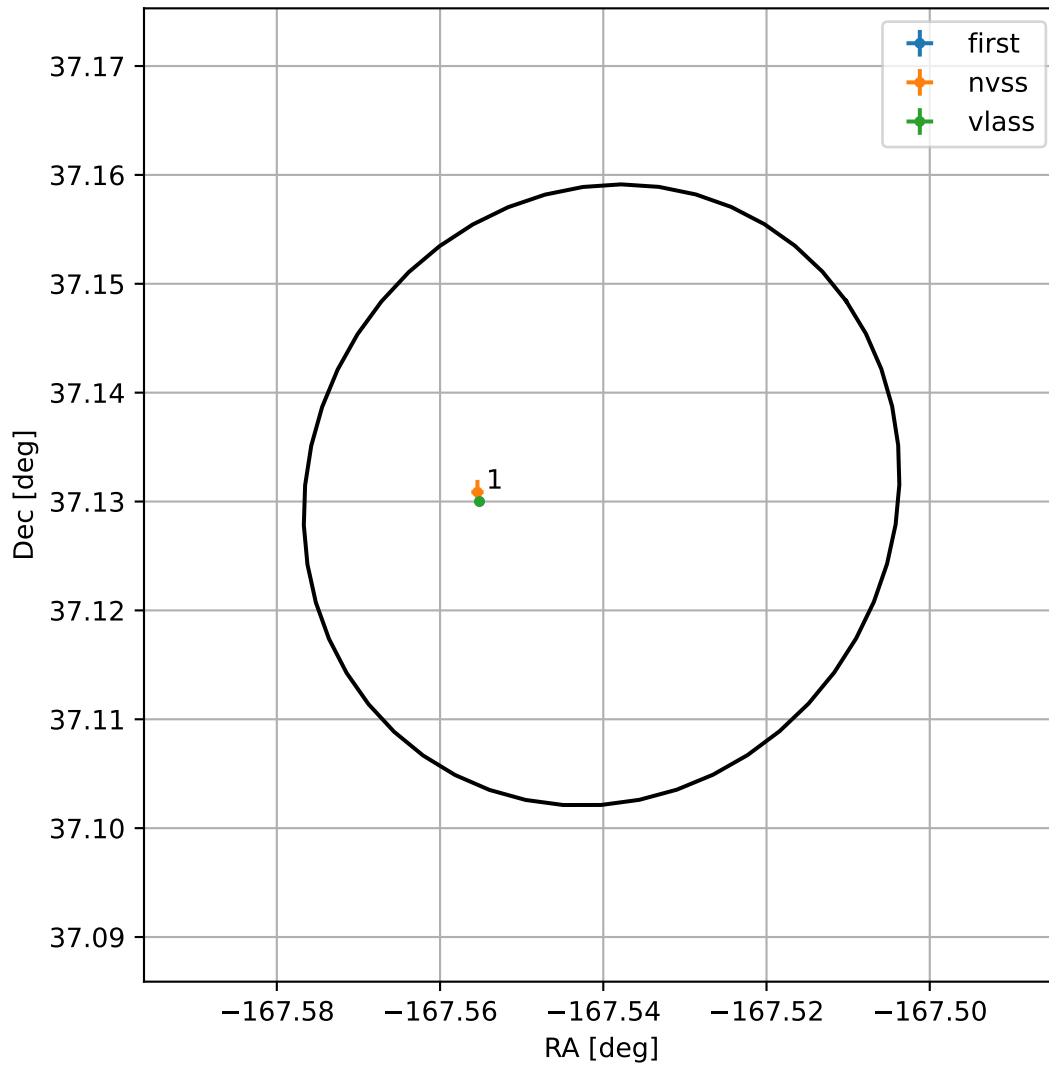
4FGL J1249.8+3707
