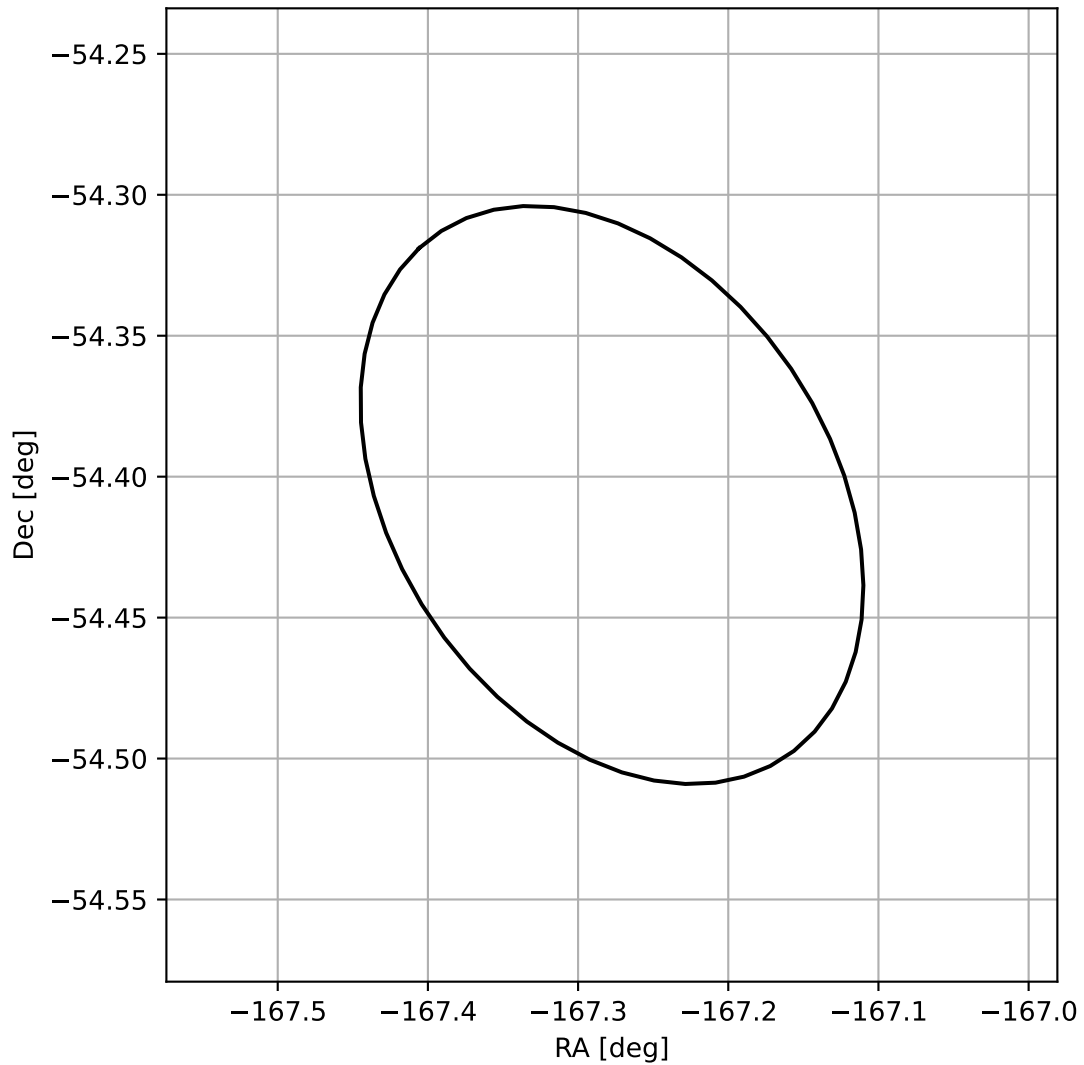
4FGL J1250.8-5424
