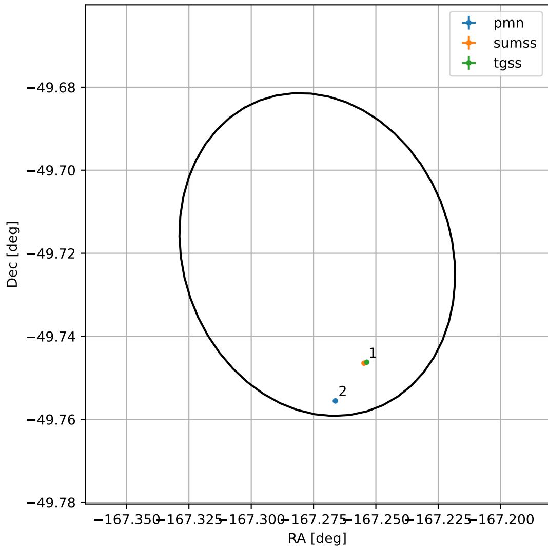
4FGL J1250.9-4943
