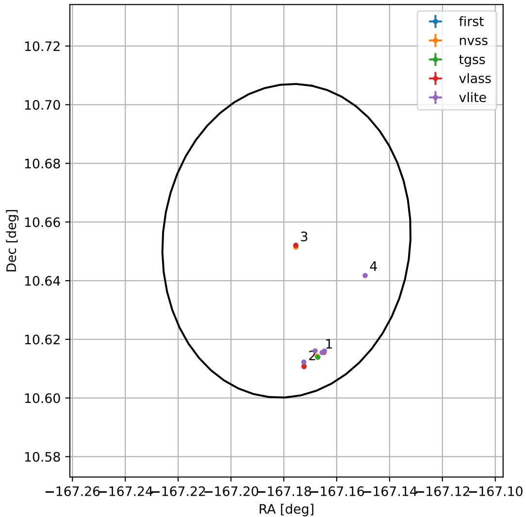
4FGL J1251.2+1039
