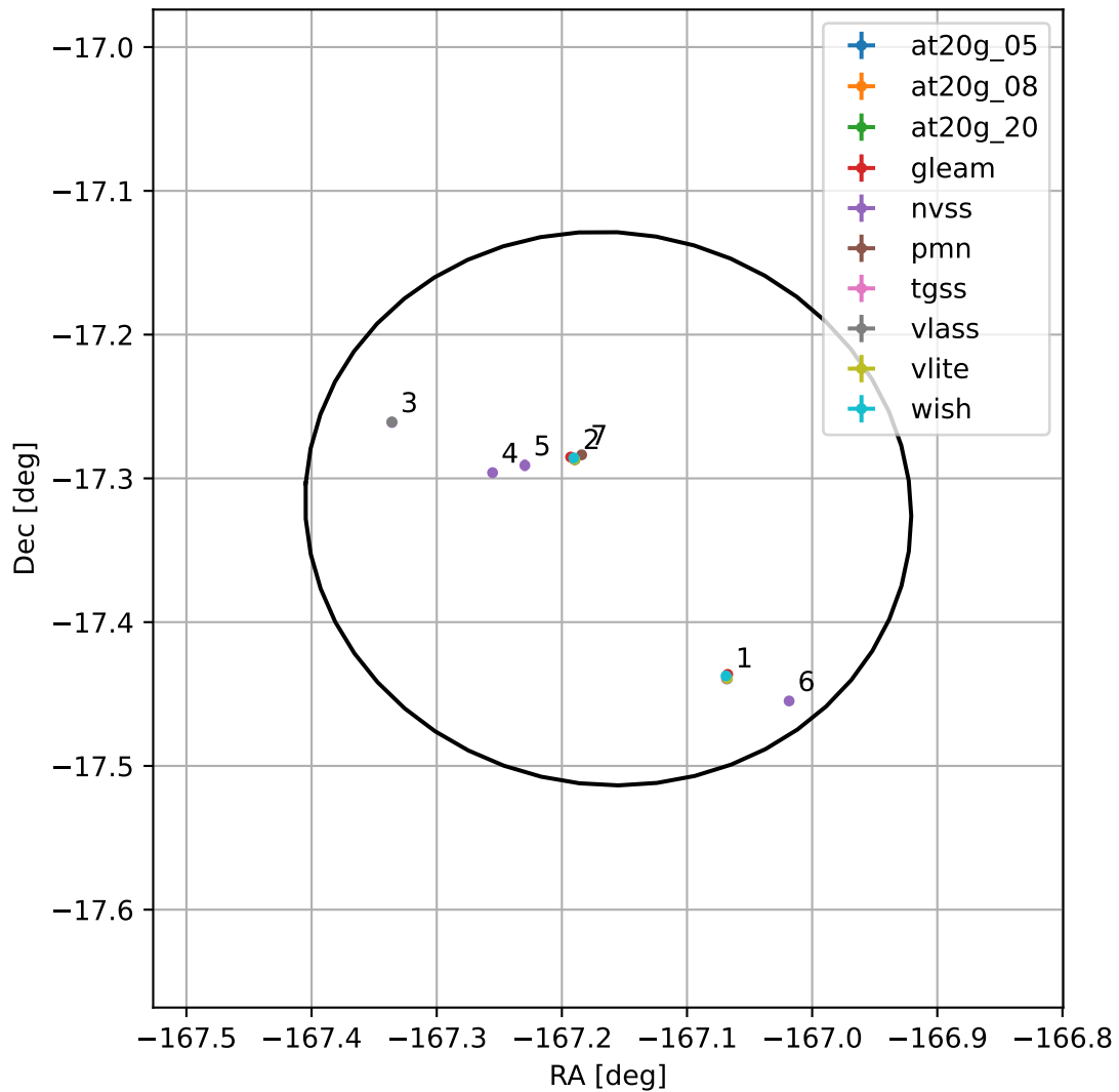
4FGL J1251.3-1719
