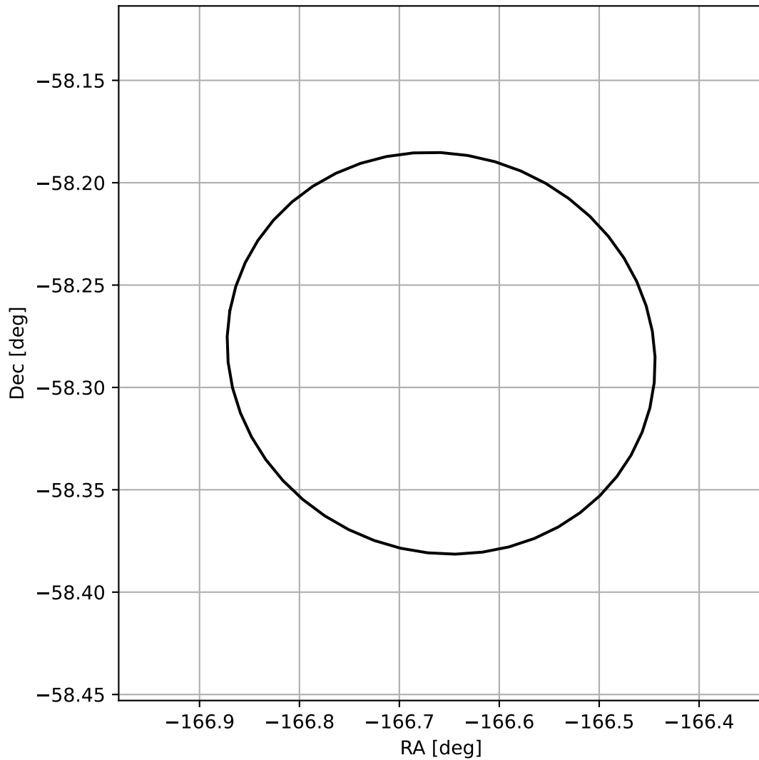
4FGL J1253.3-5816
