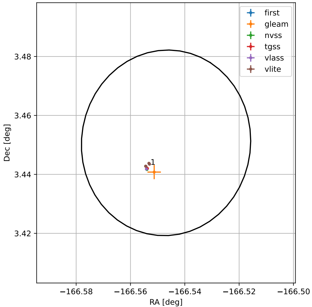
4FGL J1253.8+0327
