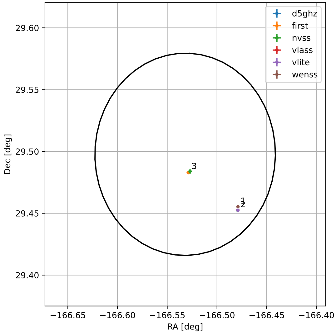
4FGL J1253.8+2929
