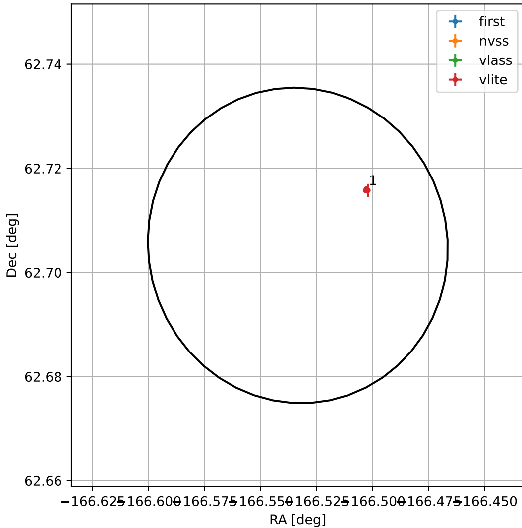
4FGL J1253.8+6242
