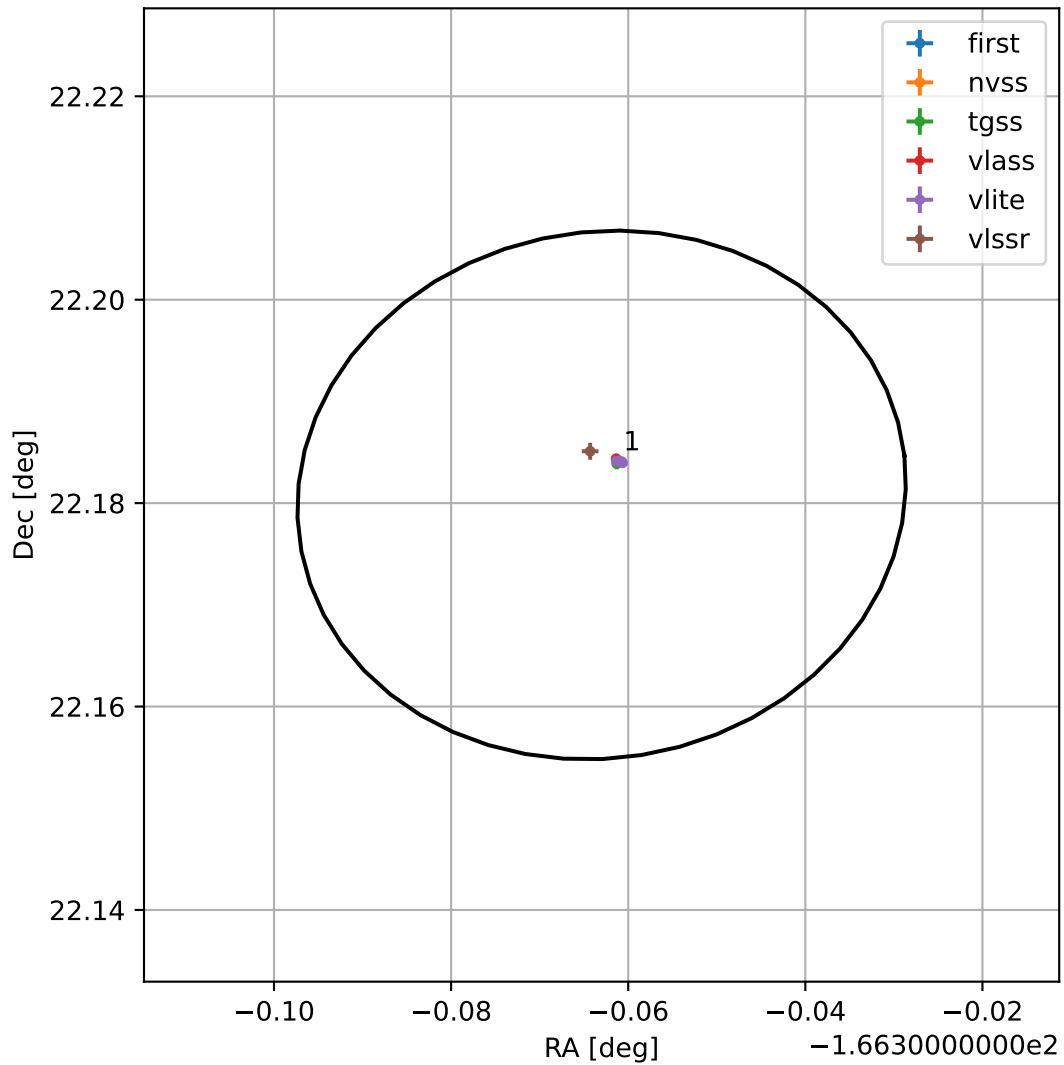
4FGL J1254.5+2210
