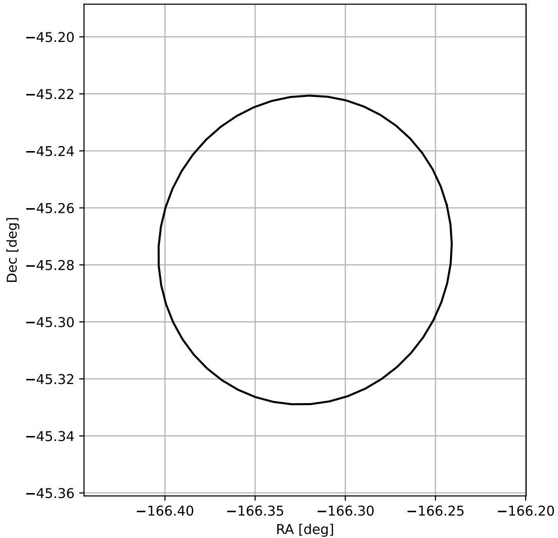
4FGL J1254.7-4516
