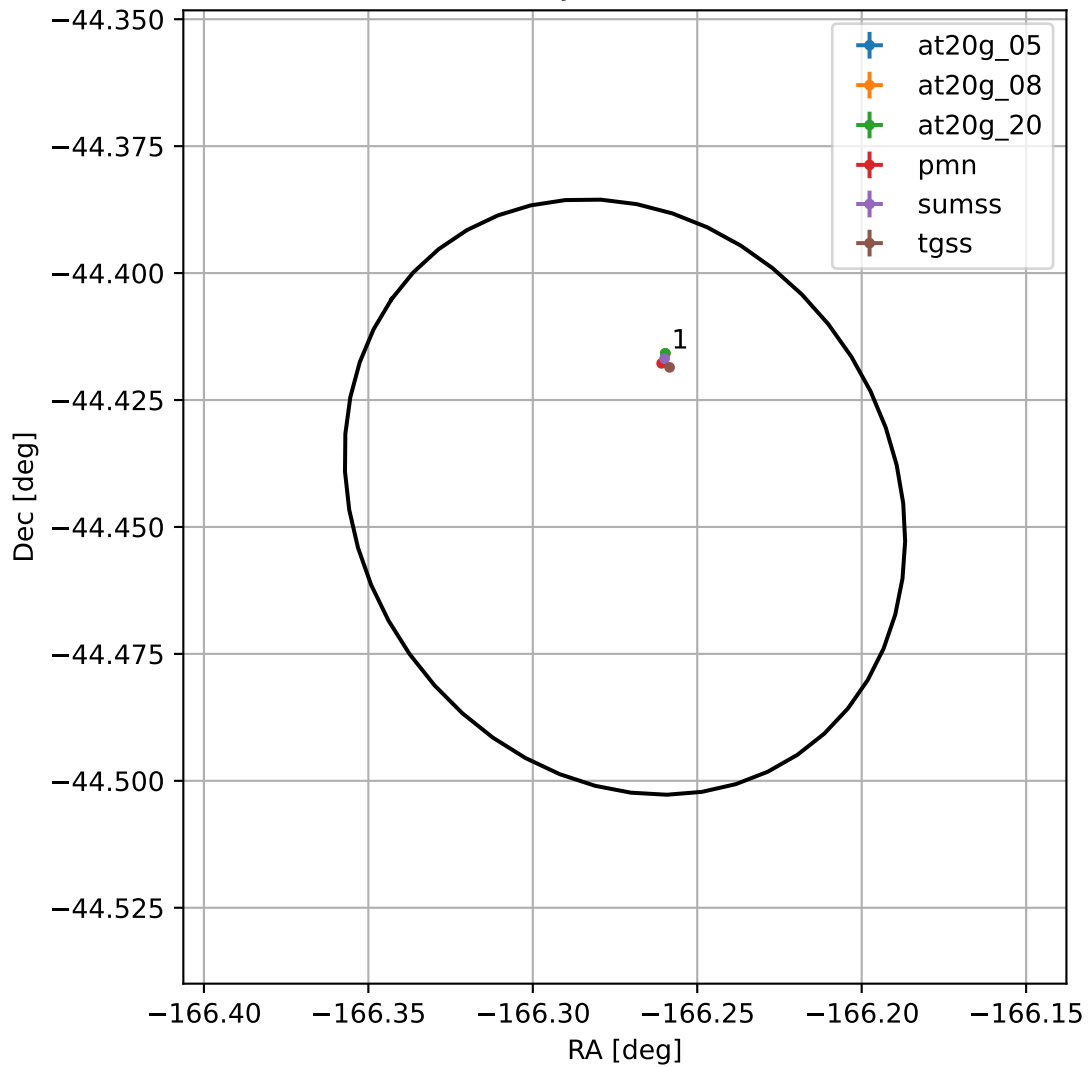
4FGL J1254.9-4426
