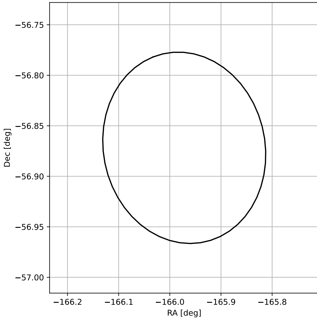
4FGL J1256.1-5652
