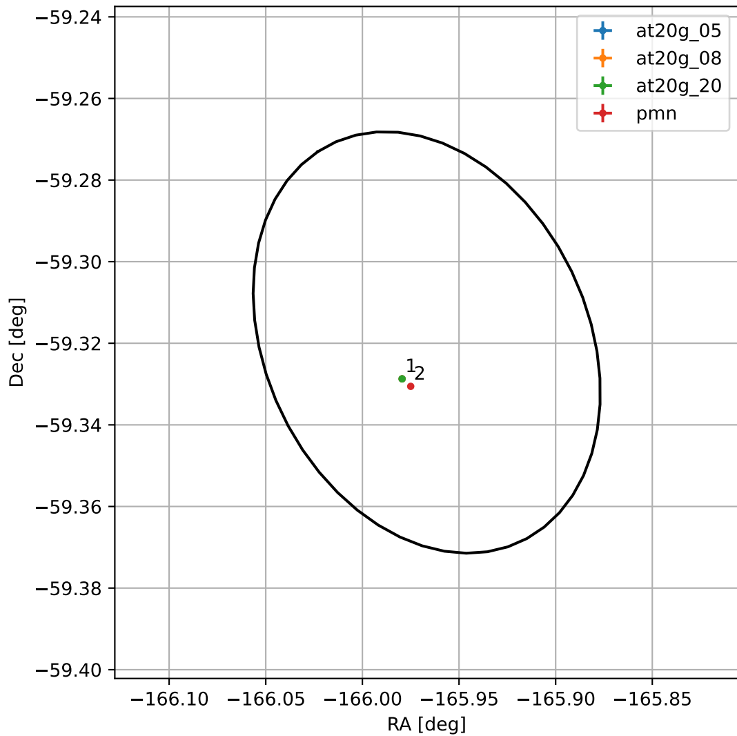
4FGL J1256.1-5919
