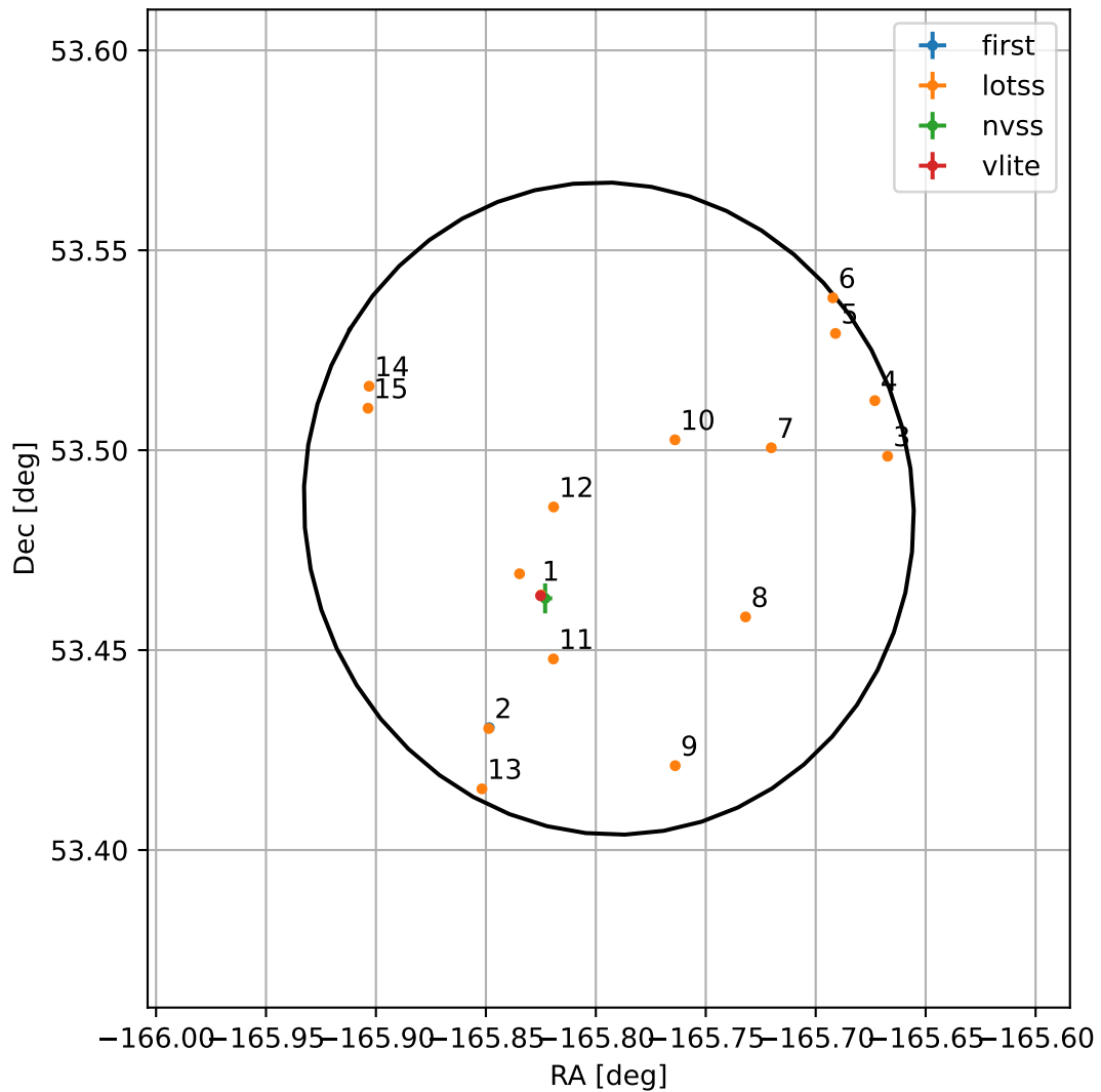
4FGL J1256.8+5329
