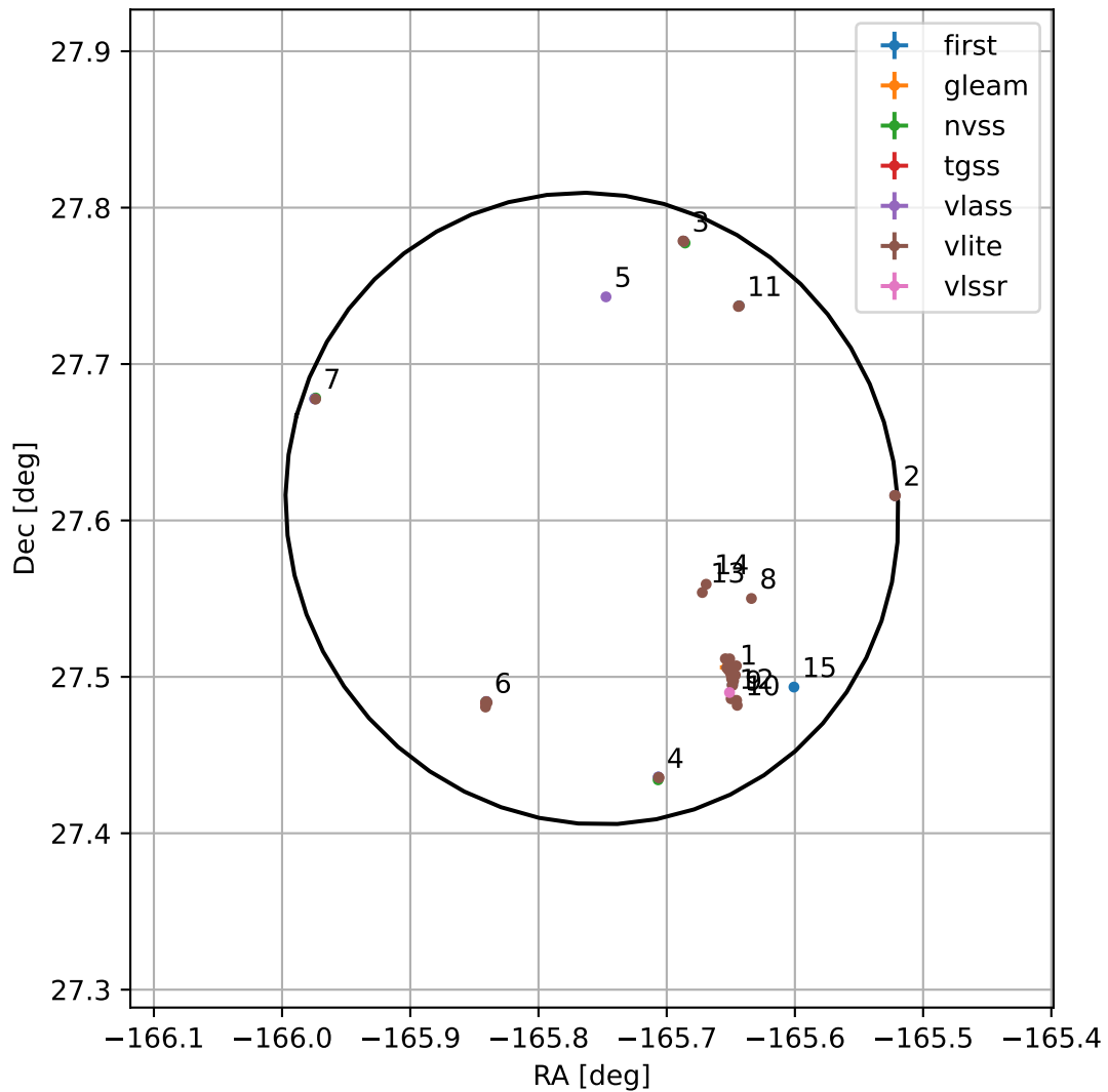
4FGL J1256.9+2736
