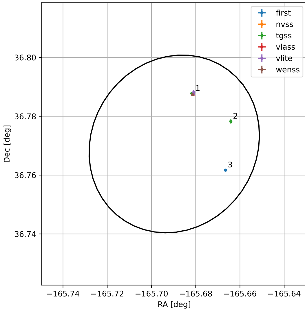
4FGL J1257.2+3646
