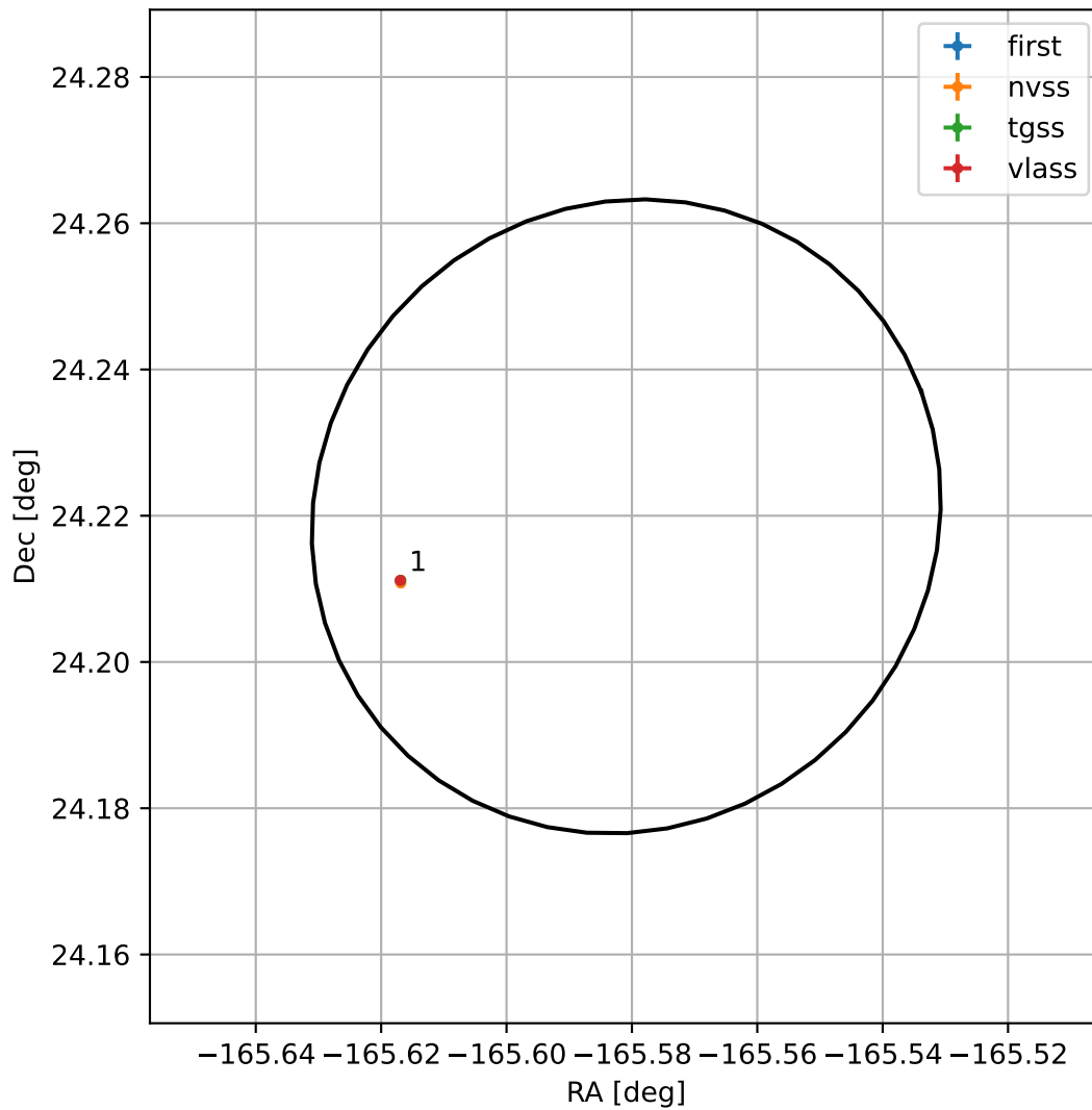
4FGL J1257.6+2413
