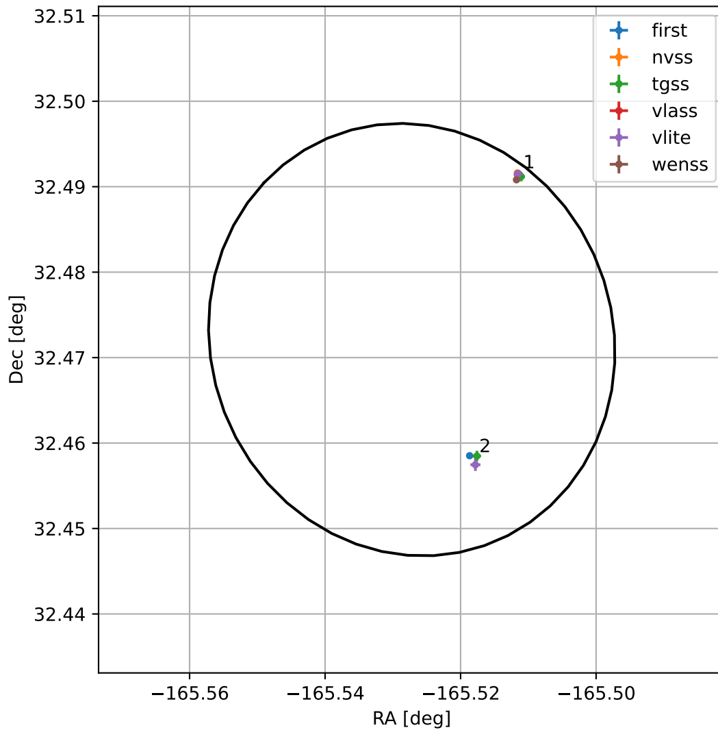
4FGL J1257.8+3228
