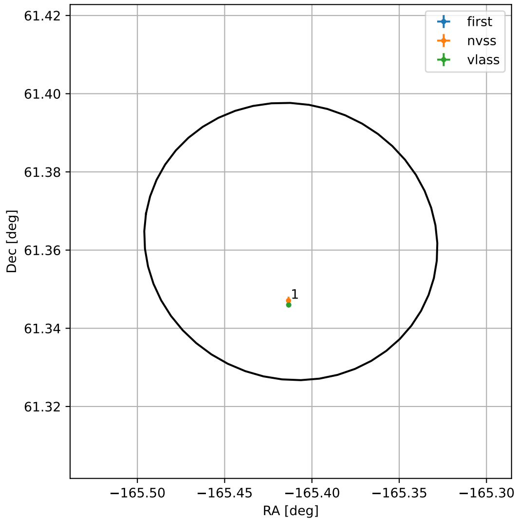
4FGL J1258.3+6121
