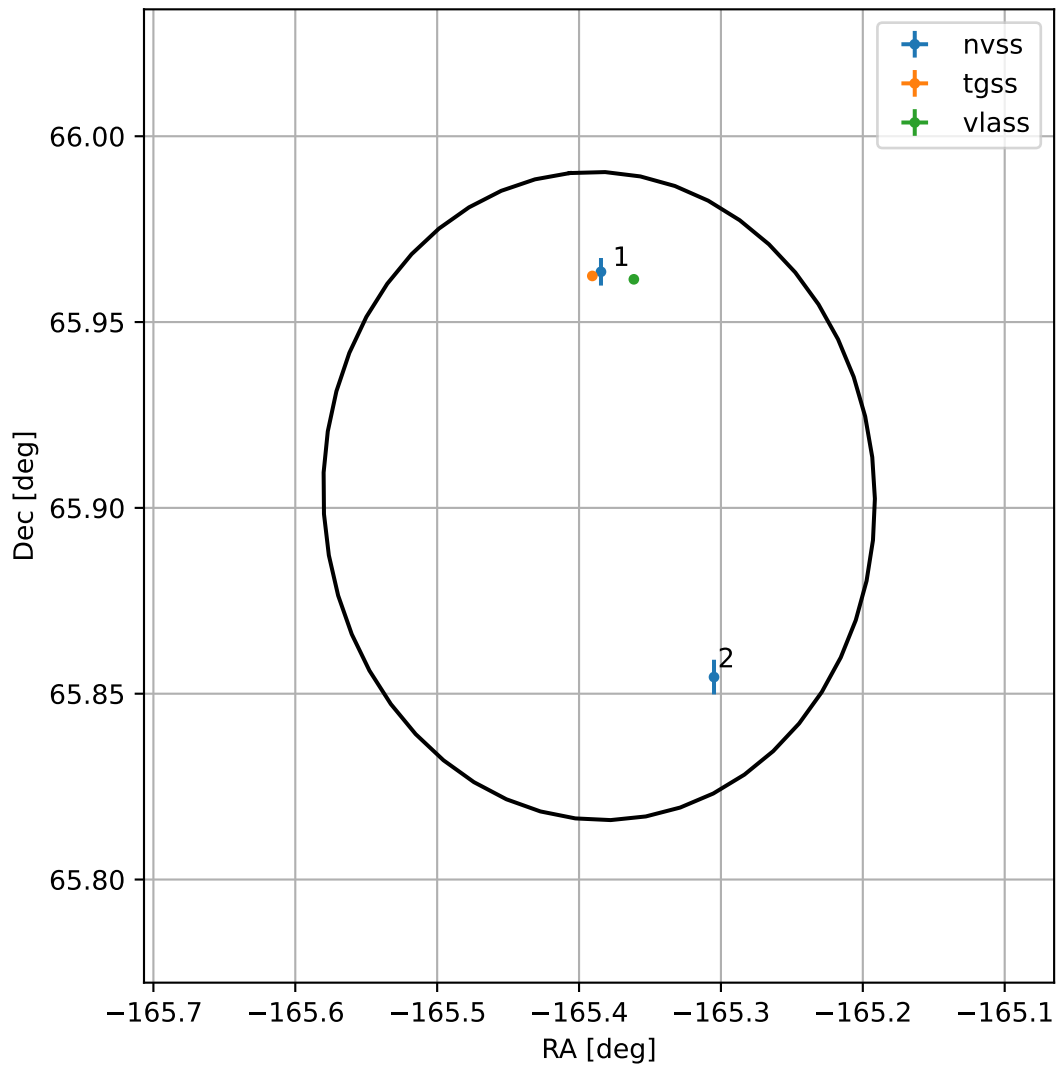
4FGL J1258.4+6554
