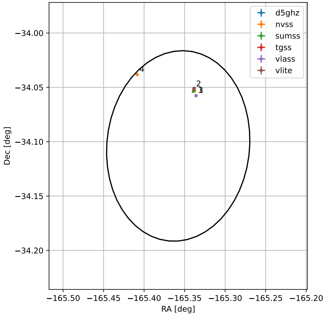
4FGL J1258.5-3406
