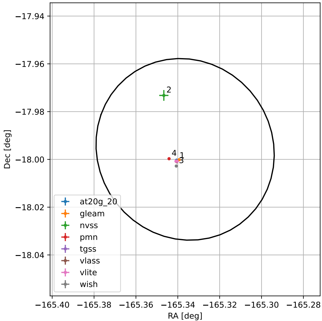
4FGL J1258.6-1759
