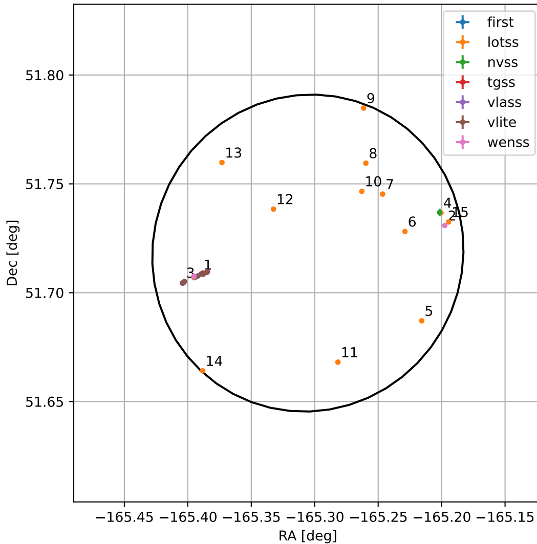
4FGL J1258.7+5143
