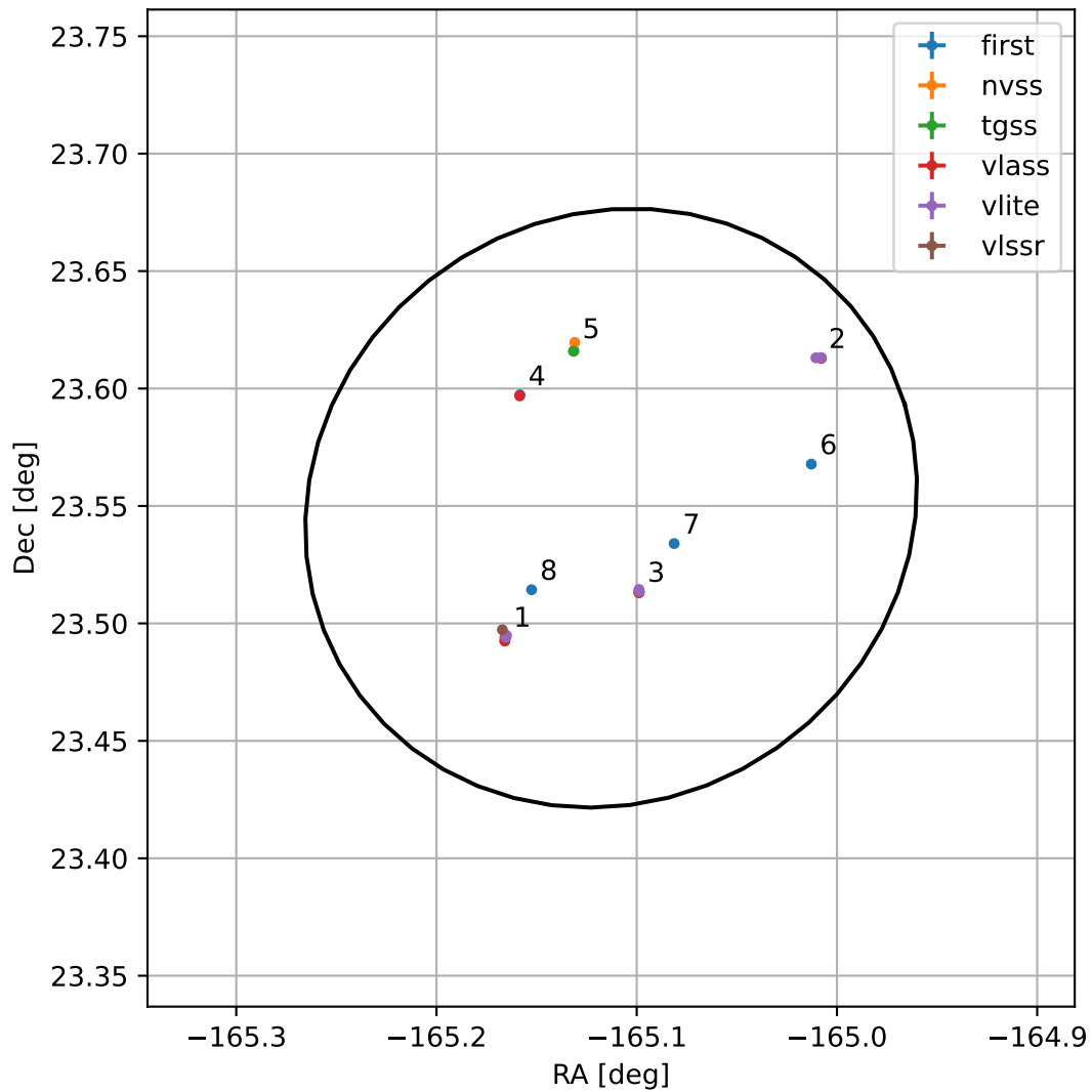
4FGL J1259.5+2332
