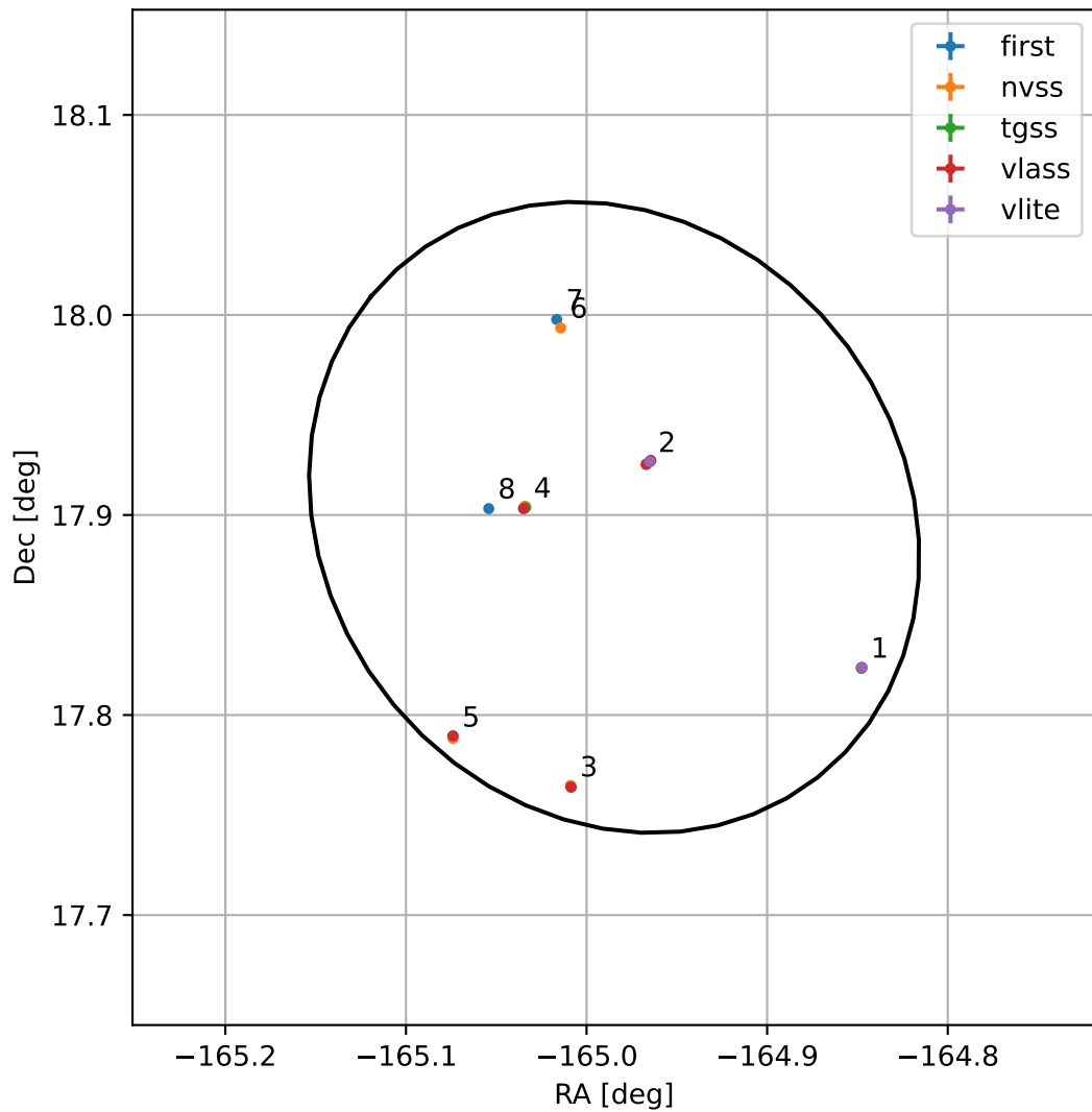
4FGL J1300.0+1753
