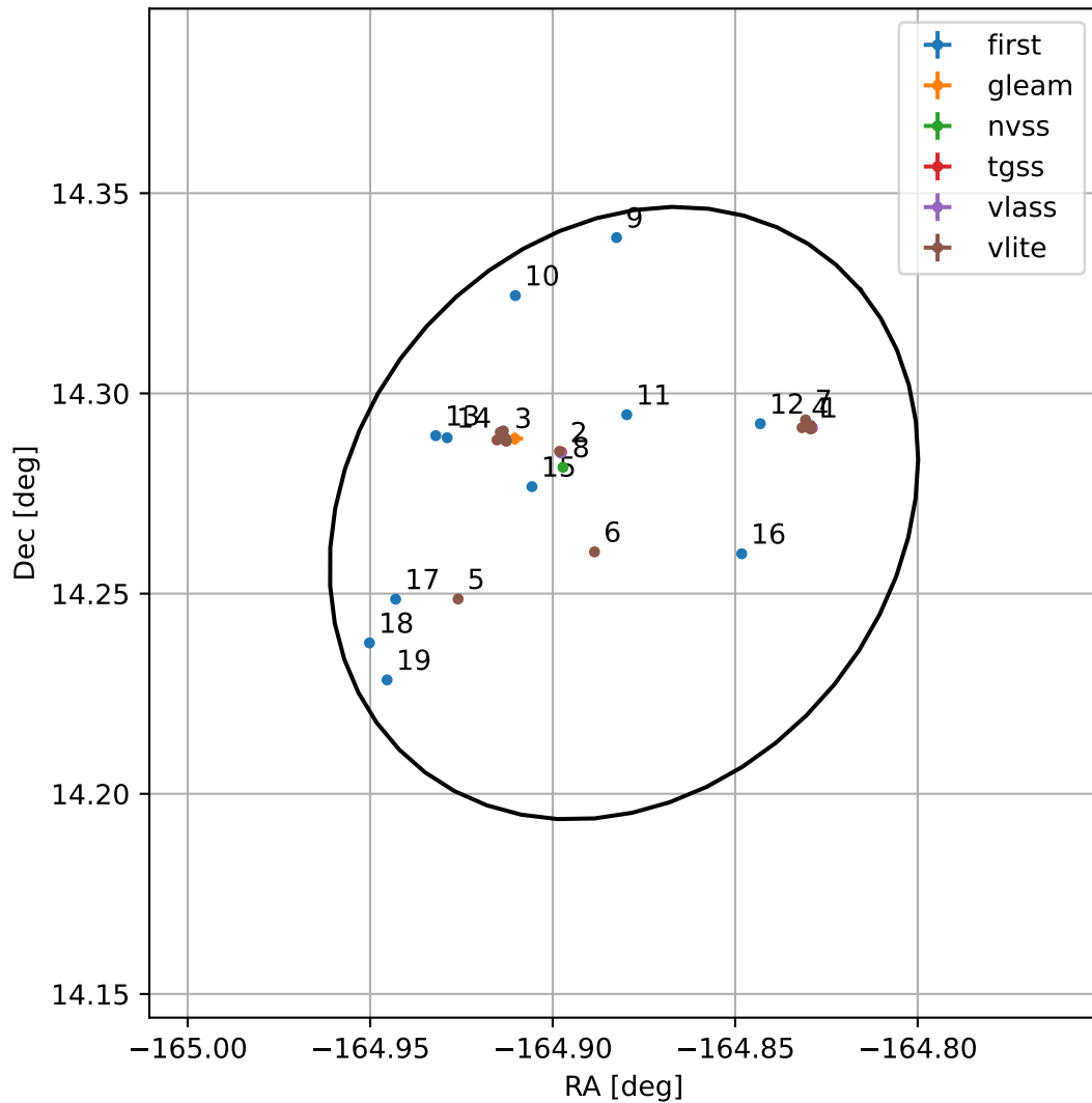
4FGL J1300.4+1416
