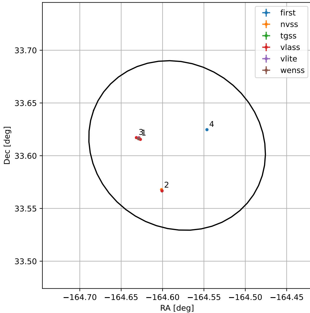
4FGL J1301.6+3336
