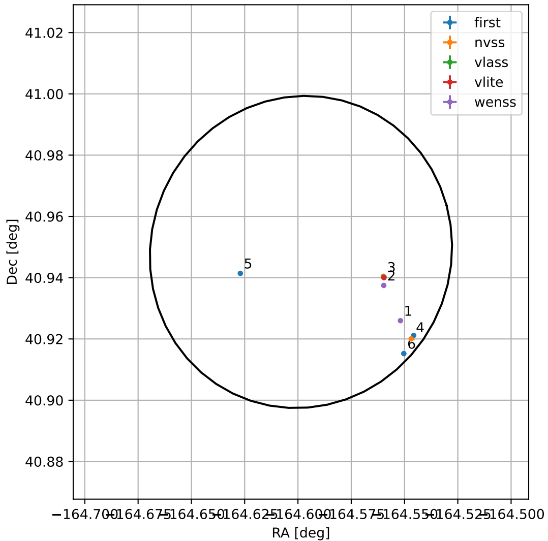
4FGL J1301.6+4056
