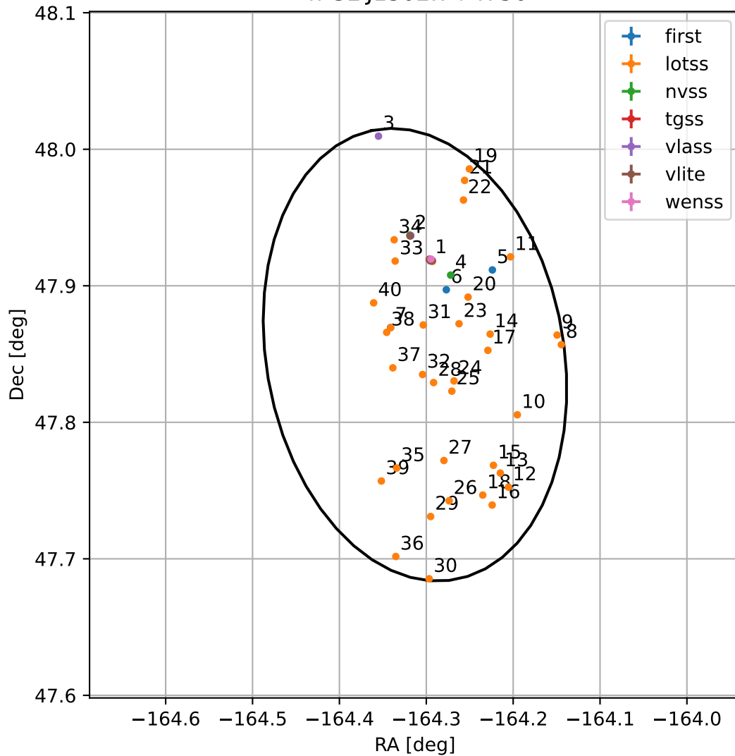
4FGL J1302.7+4750
