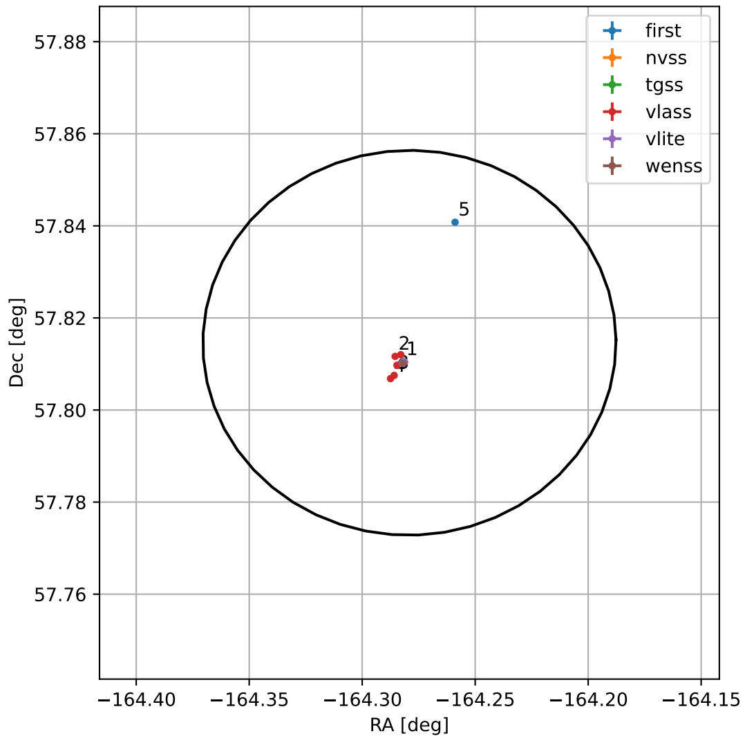
4FGL J1302.8+5748
