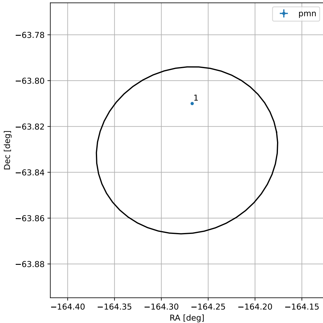
4FGL J1302.9-6349
