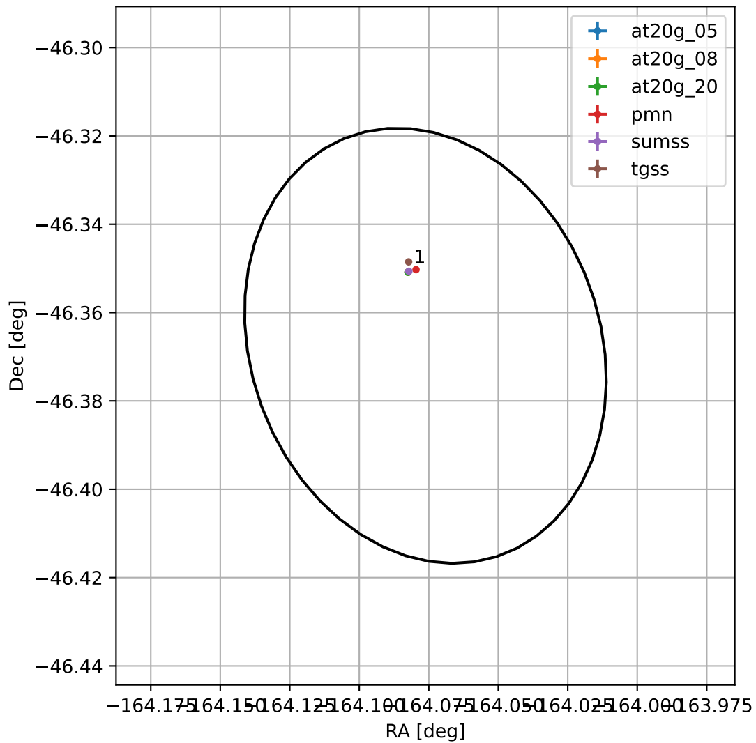
4FGL J1303.6-4622
