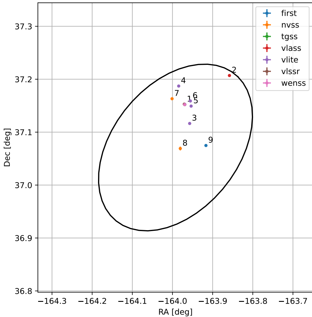
4FGL J1304.0+3704
