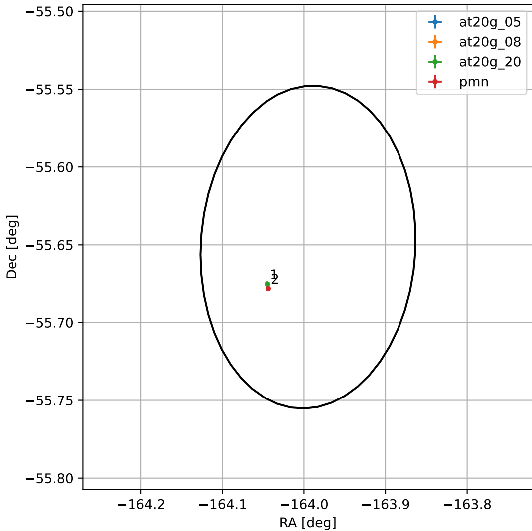
4FGL J1304.0-5539
