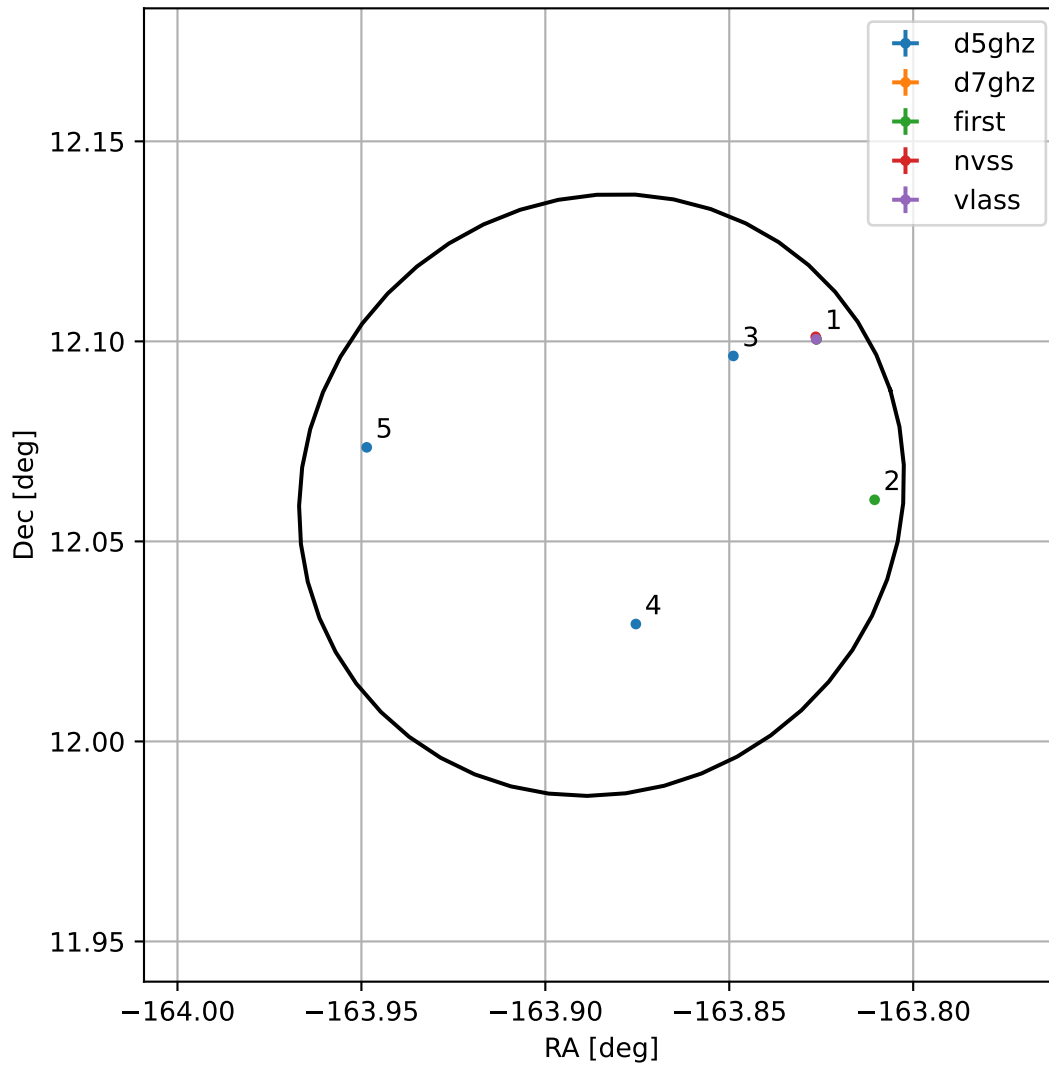
4FGL J1304.4+1203
