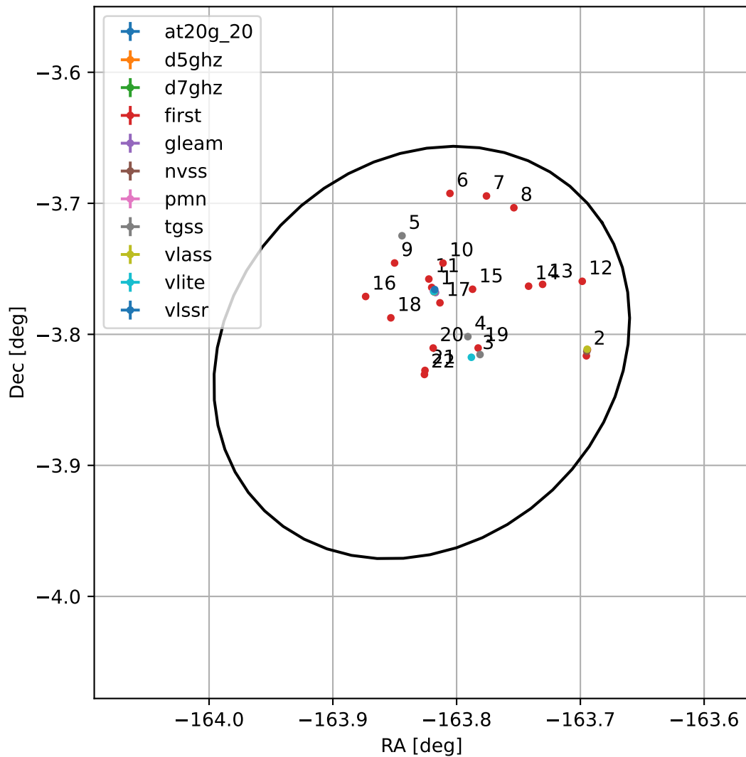
4FGL J1304.6-0348
