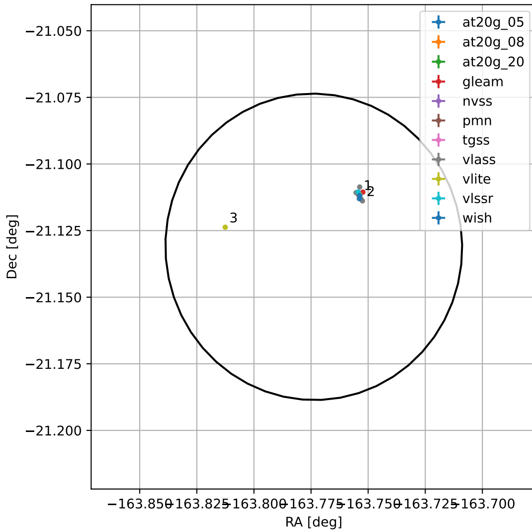
4FGL J1304.9-2107
