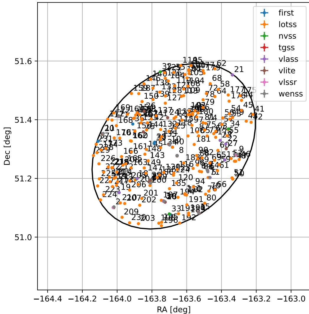
4FGL J1305.3+5118
