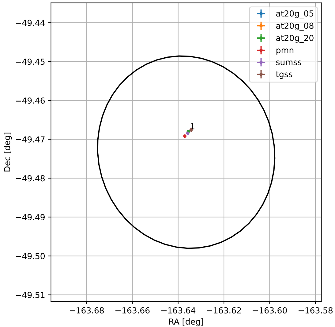
4FGL J1305.4-4928
