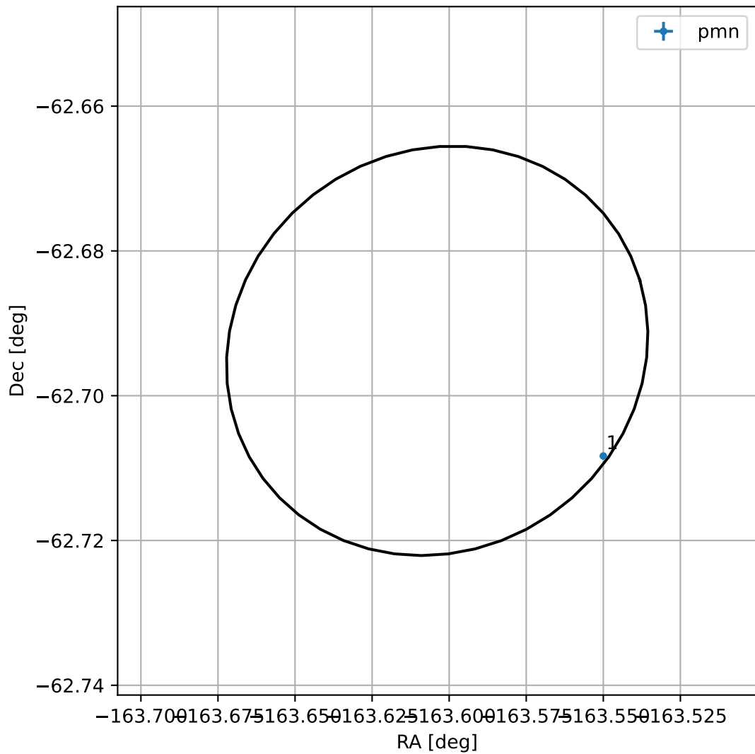
4FGL J1305.5-6241
