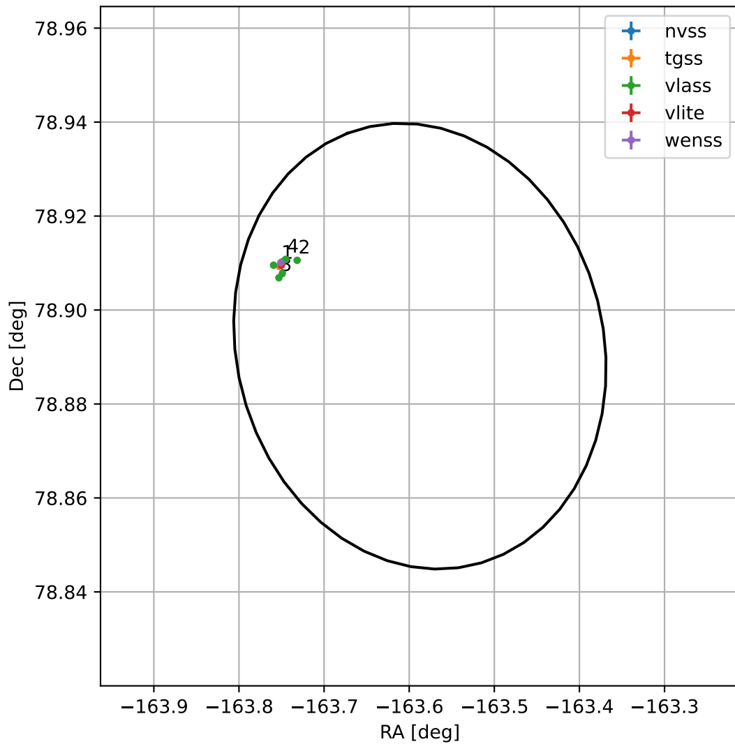
4FGL J1305.6+7853
