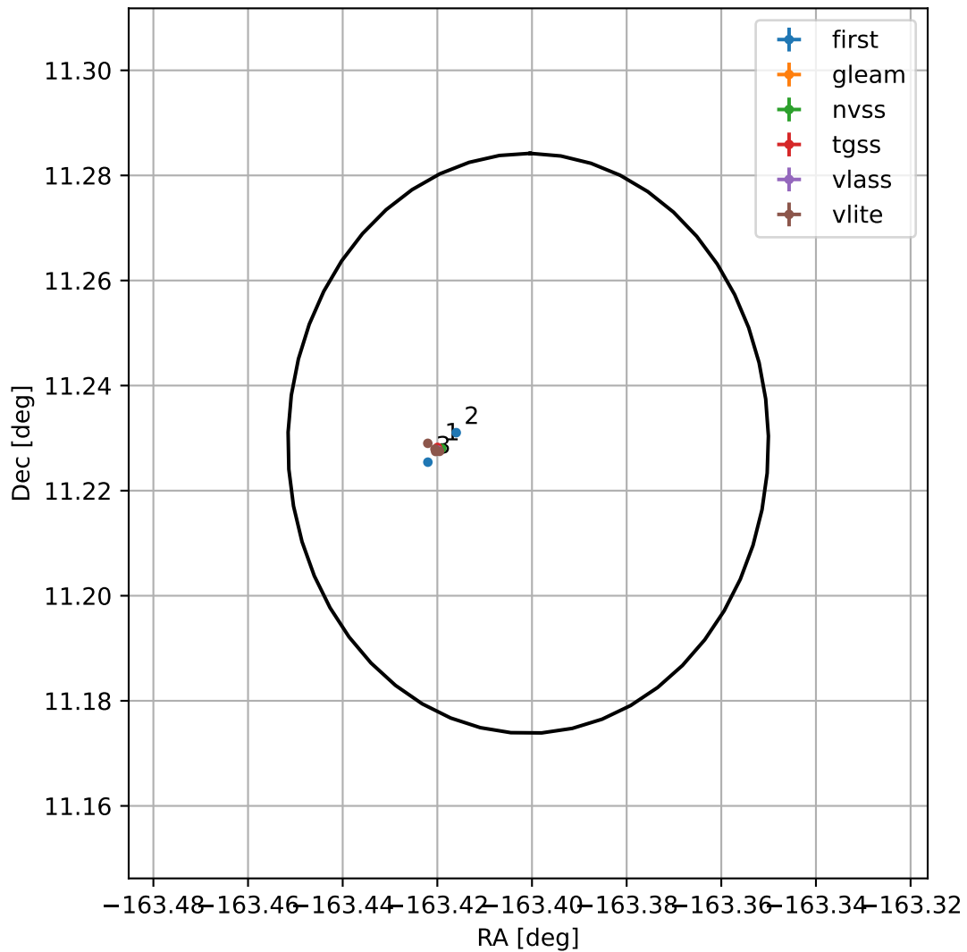
4FGL J1306.3+1113
