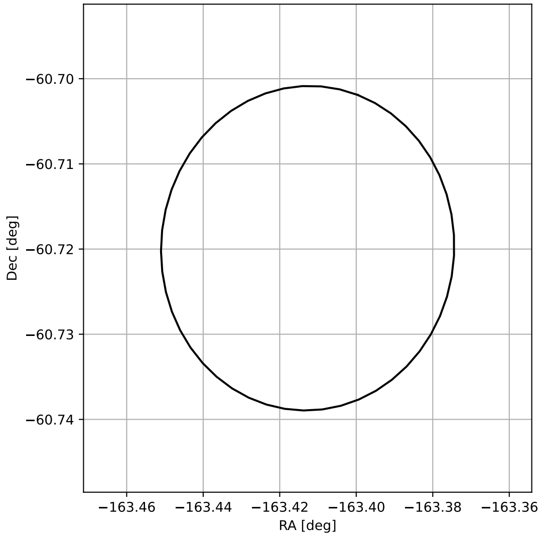
4FGL J1306.3-6043
