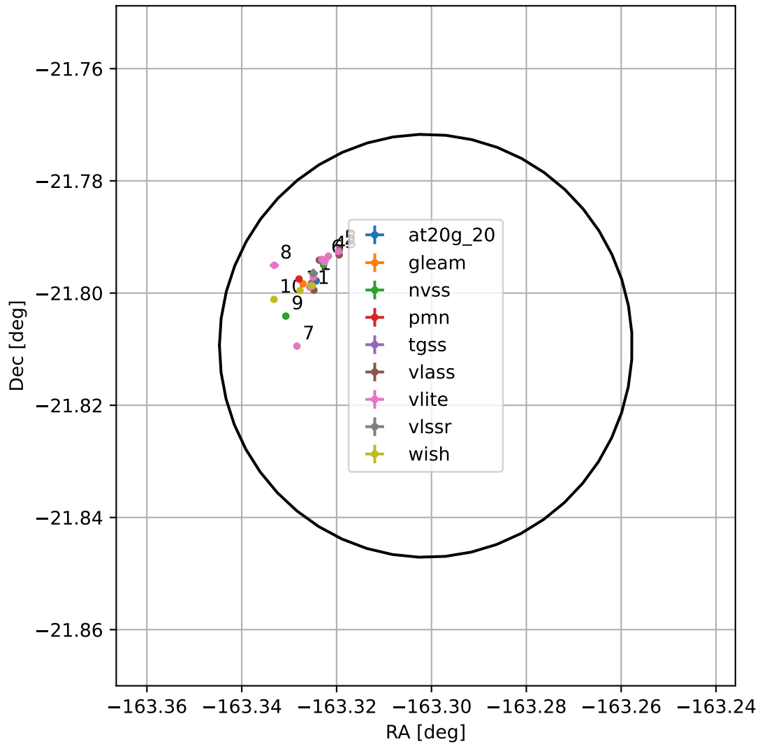
4FGL J1306.7-2148
