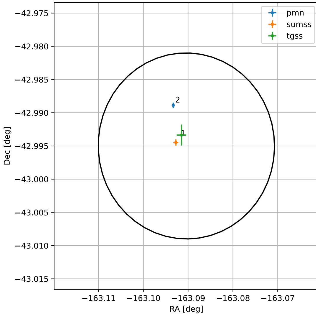
4FGL J1307.6-4259
