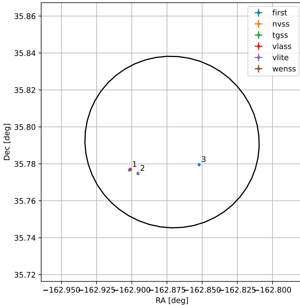
4FGL J1308.5+3547
